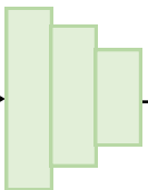
Text Backbone
