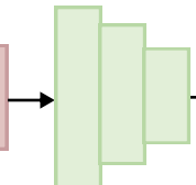
Image Backbone
